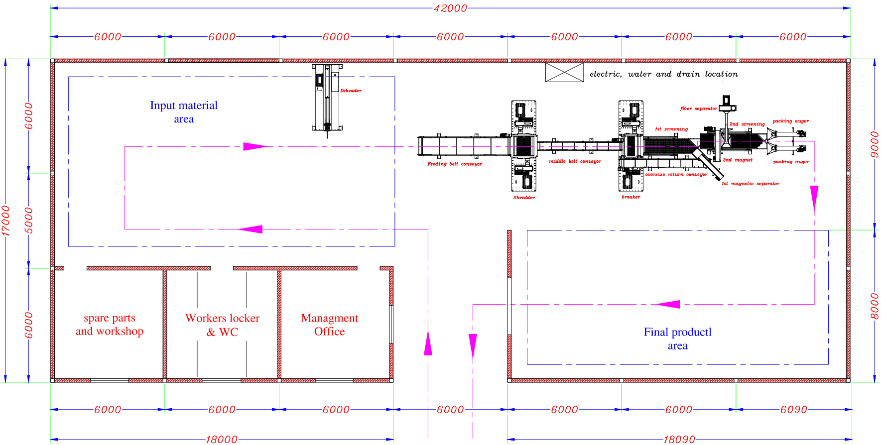
plant layout for tire recycling line 500 kg/hr
